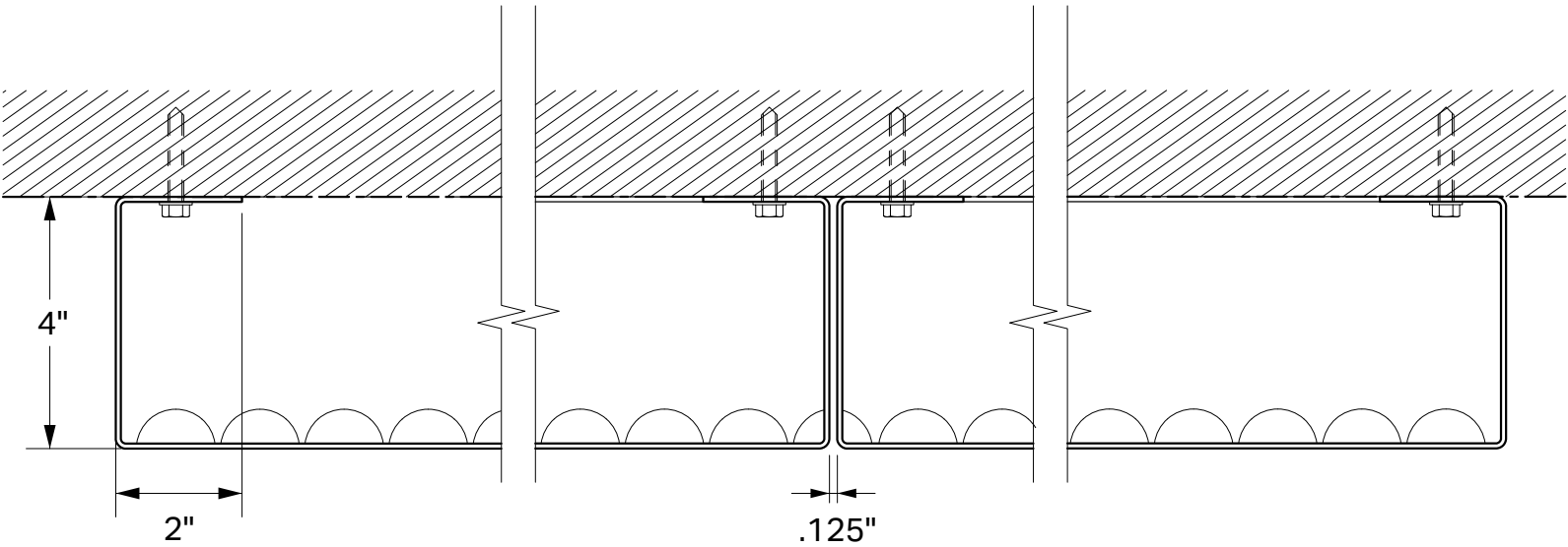
B-B Plan Section 1" = 3"
