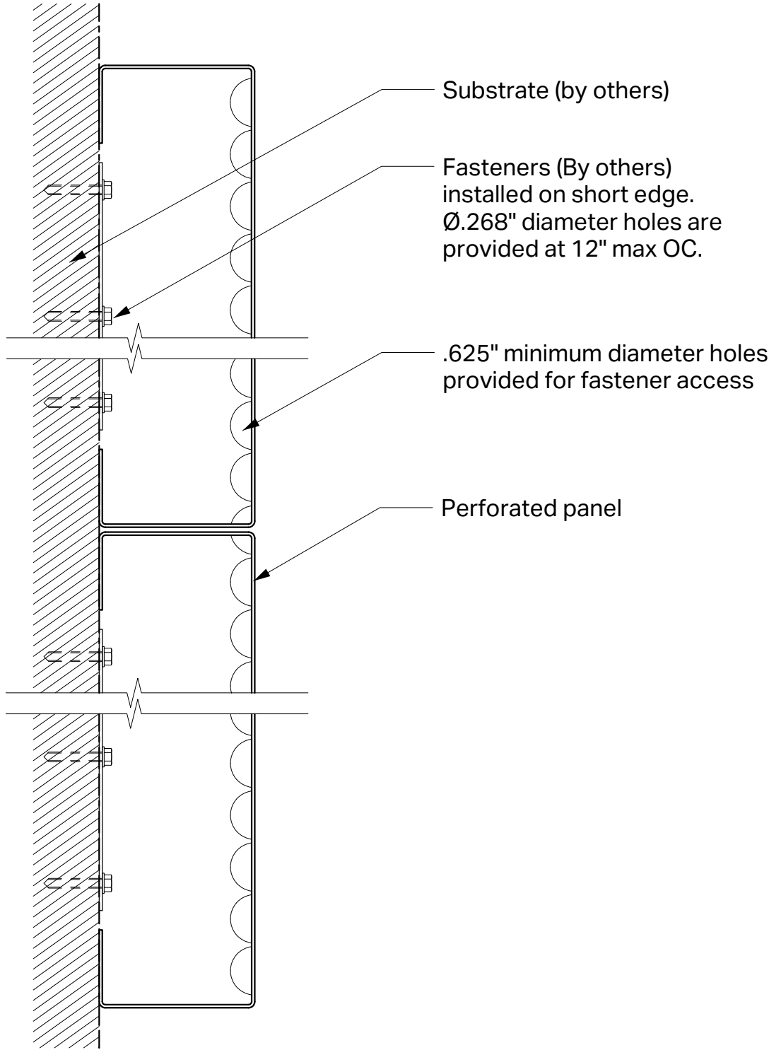
A-A Vertical Section
