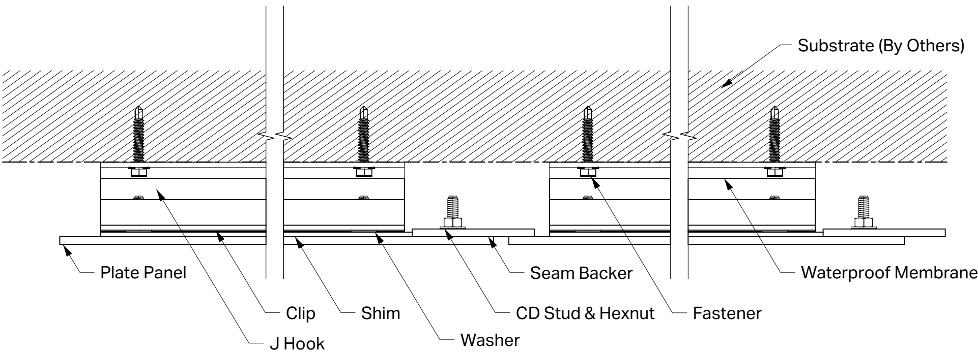
B-B Plan Section
