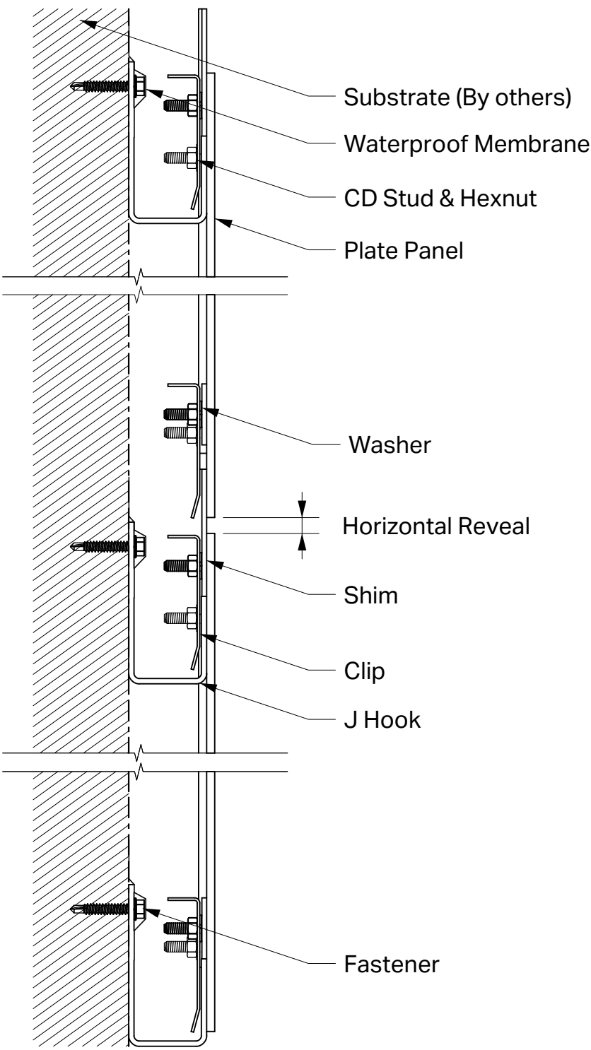
A-A Vertical Section
