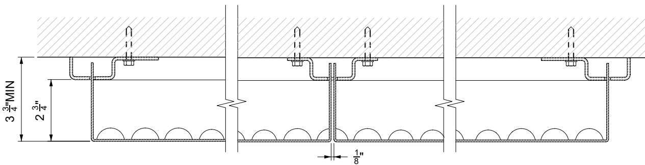
Plan Section (B-B)
