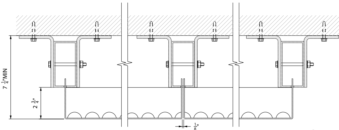
Plan Section (B-B)
