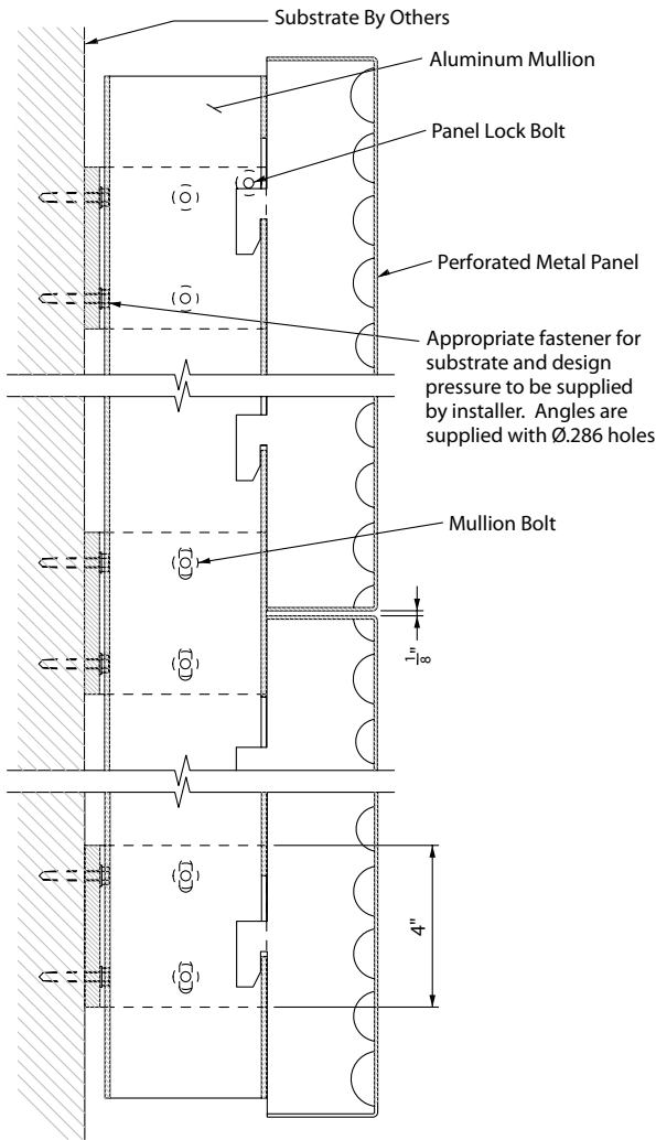
Vertical Section (A-A)
