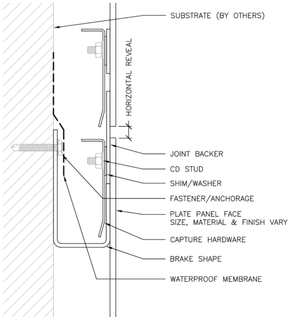
Horizontal Joint - Elevation Section
