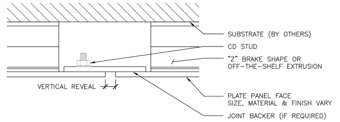
Vertical Joint - Plan Section
